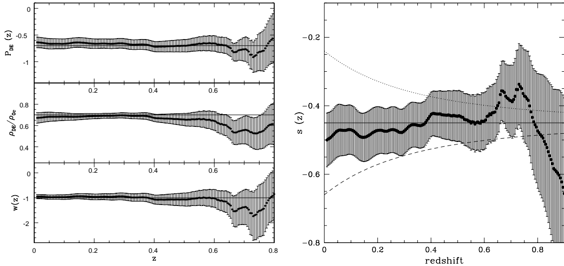
FIGURE 2. Dark energy pressure (top left panel), energy density (middle left panel), and equation of state (bottom left panel), and the dark energy indicator (right panel) as functions of redshift for a combined sample of supernovae and radio galaxies; from Daly et al. (2008).
