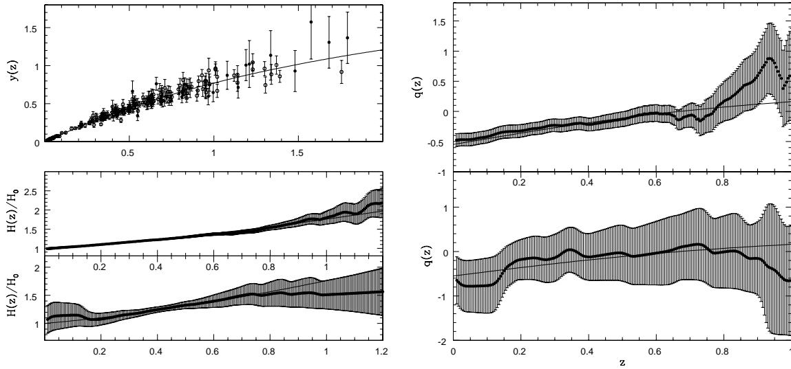
FIGURE 1. Dimensionless coordinate distances (filled symbols indicate radio galaxies and open symbols indicate supernovae), H(z) for supernovae (middle left panel) and radio galaxies (bottom left panel), and q(z) for supernovae (top right panel) and radio galaxies (bottom right panel); from Daly et al. (2008).
