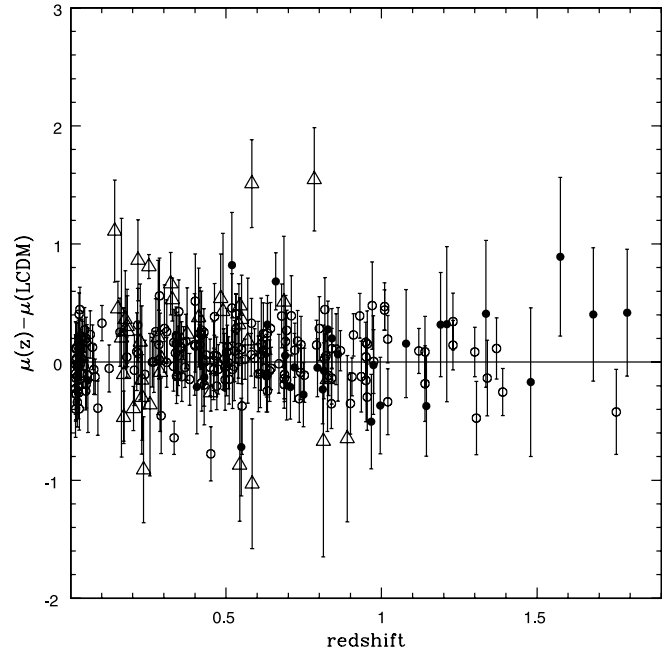
FIG. 1.—Difference between the distance modulus to the source and that expected in a standard LCDM model with \Omega_m = 0.3 and \Omega_\Lambda = 0.7 . Open circles represent the 192 supernovae of Davis et al. (2007), filled circles represent the 30 radio galaxies of Daly et al. (2008), and open triangles represent the 38 clusters of Bonamente et al. (2006).
